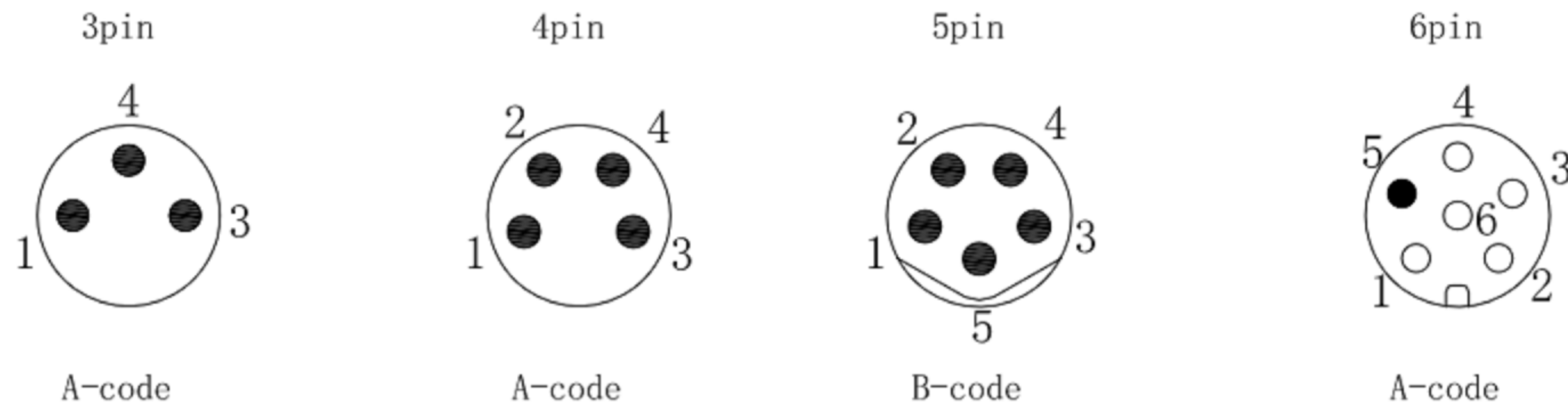
Pin assignment front view/针位分布前视图
